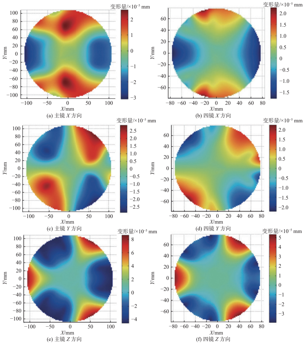
图 14 主、四镜面形云图 Fig. 14 Cloud atlas of surface shape for primary-fourth mirror
